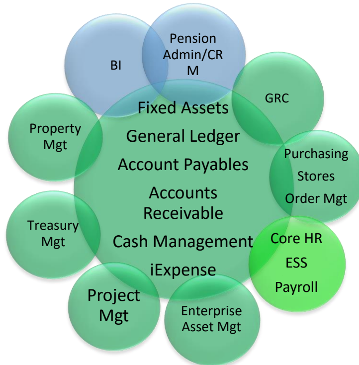
Figure 1: Modules Implemented
